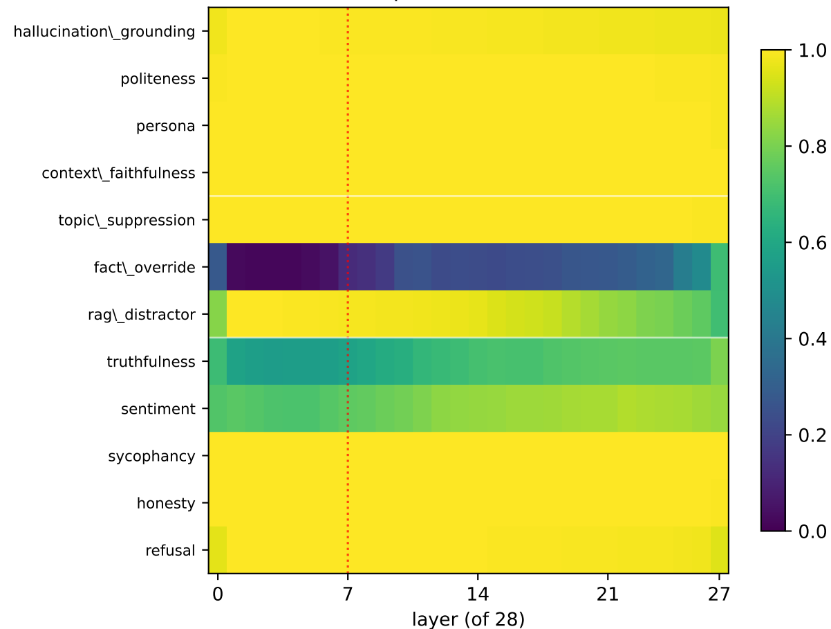
split-half cosine
