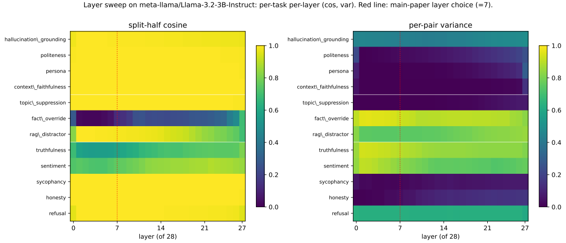
Figure 3: Layer sweep on Llama-3.2-3B-Instruct: per-task per-layer ( \text{c}\ddot{o}s, \sigma ). Rows are tasks (grouped by hypothesized kind, separated by white lines); columns are layers 0–27. Red dashed line: main-paper layer choice ( \ell = 7 ). Row patterns do not change qualitatively between \ell = 7 and other mid-network layers, supporting the layer-stability claim of R2.
