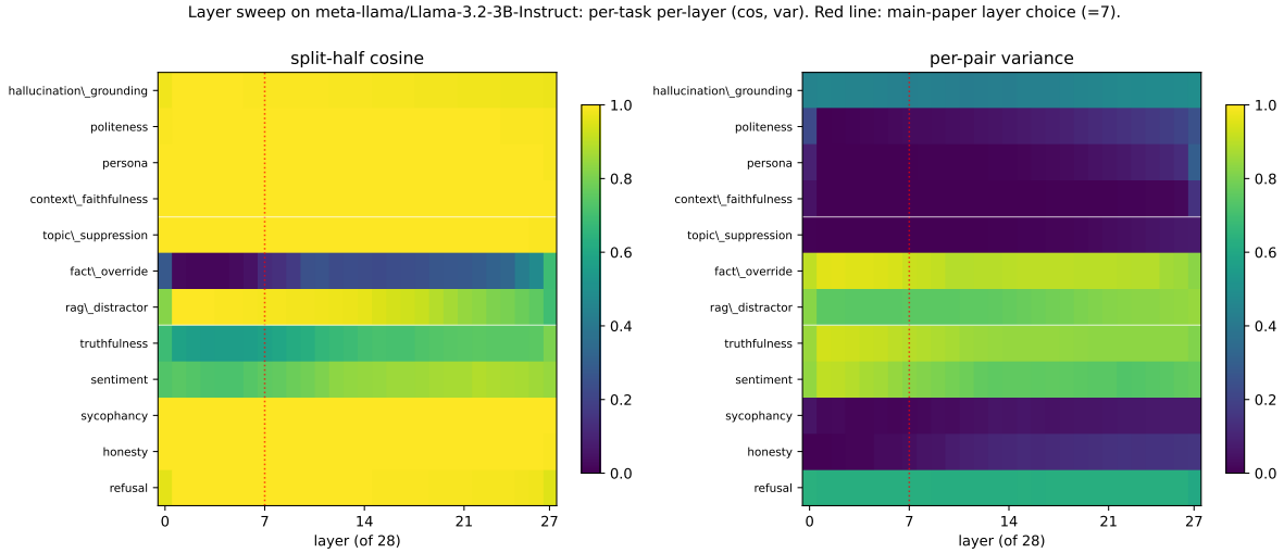
Figure 3: Layer sweep on Llama-3.2-3B-Instruct: per-task per-layer ( \bar{\cos}, \sigma ). Rows are tasks (grouped by hypothesized kind, separated by white lines); columns are layers 0–27. Red dashed line: main-paper layer choice ( \ell = 7 ). Row patterns do not change qualitatively between \ell = 7 and other mid-network layers, supporting the layer-stability claim of R2.
