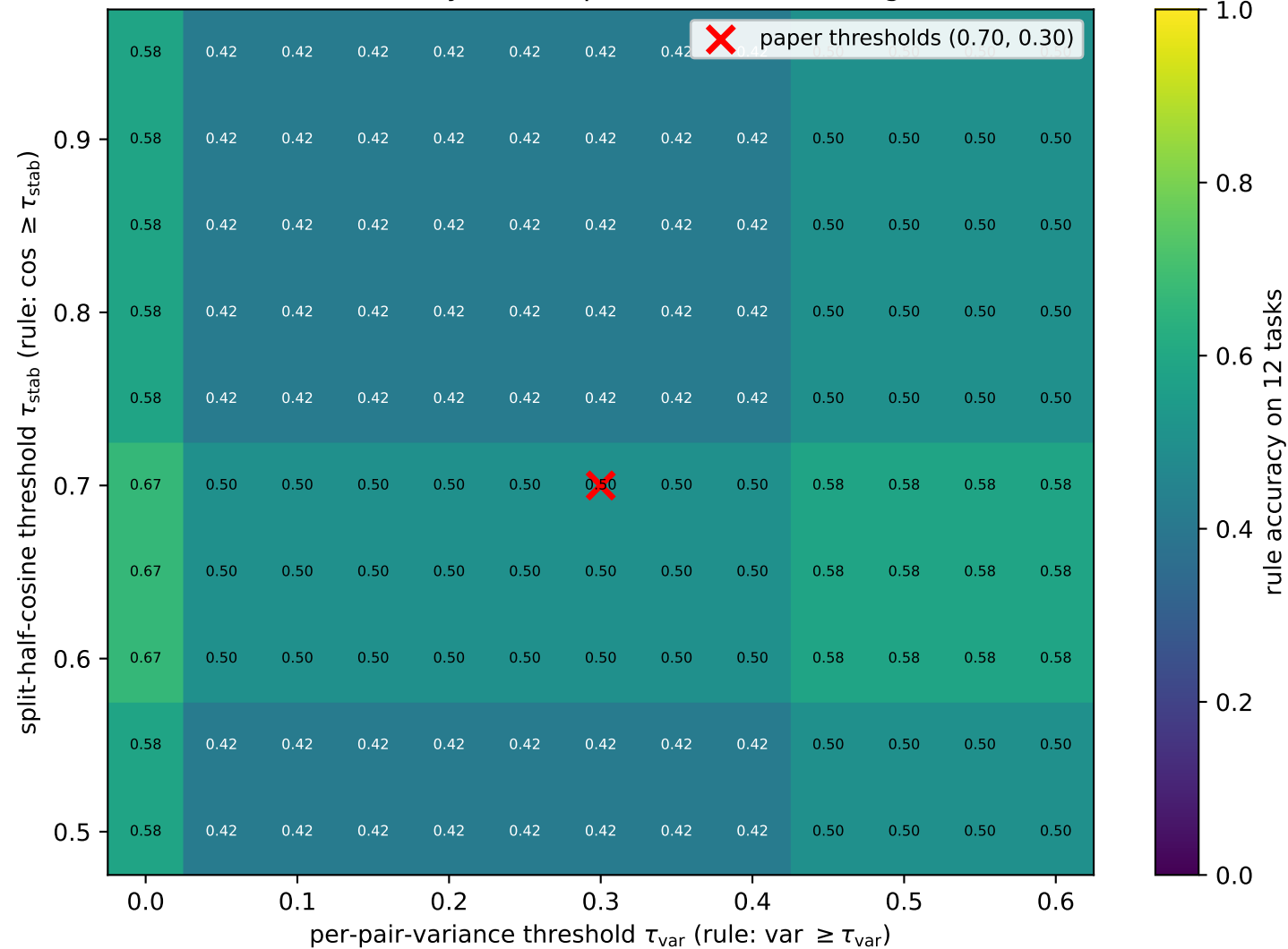
Rule-accuracy heatmap over the threshold grid
