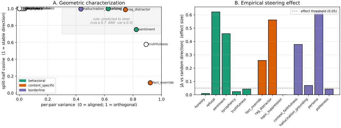
Figure 1: The 12-task taxonomy on Llama-3.2-3B-Instruct. A. Geometric scatter: per-pair variance ( x ) vs. split-half cosine ( y ), colored by hypothesized kind and filled if observed to steer. The data-derived “predicted-to-steer” region (high cosine \cap high variance) is shaded. B. Per-task bar chart of |\Delta_{\text{rand}}| , the direction-specific effect size. Dashed line is the steers/no-steers threshold (0.05). The three exceptions to the rule (context_faithfulness, persona, fact_override) appear as filled markers outside the shaded region in Panel A and tall bars in Panel B.
