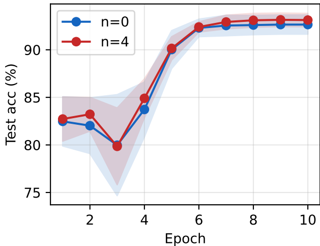
(b) Held-out test accuracy
