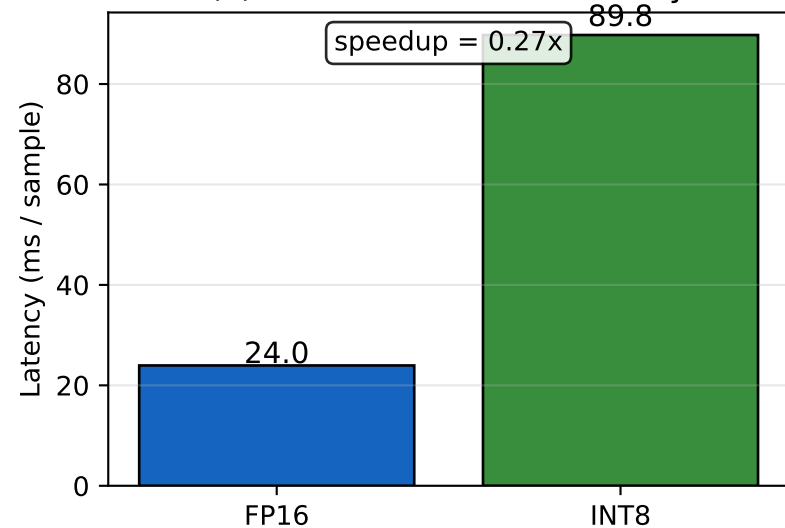
(a) NVIDIA RTX A4000 latency
