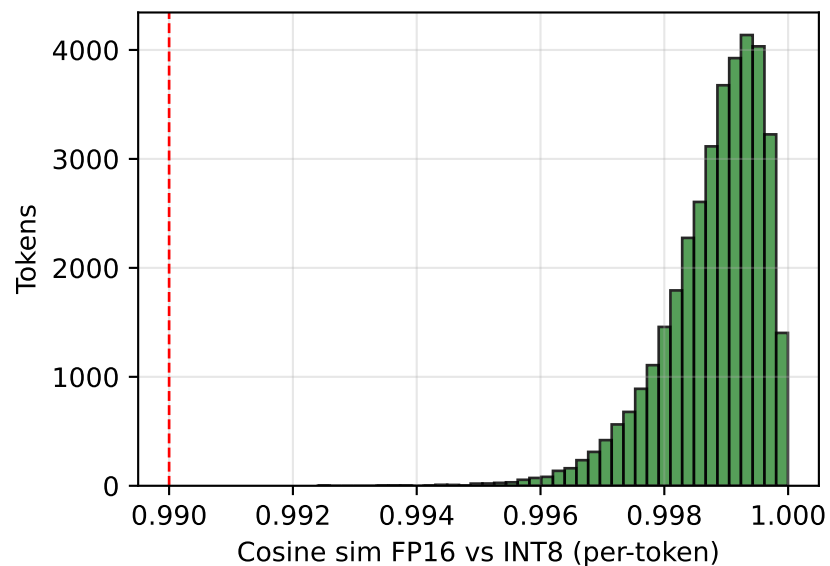
(b) Token-state agreement mean = 0.9988
