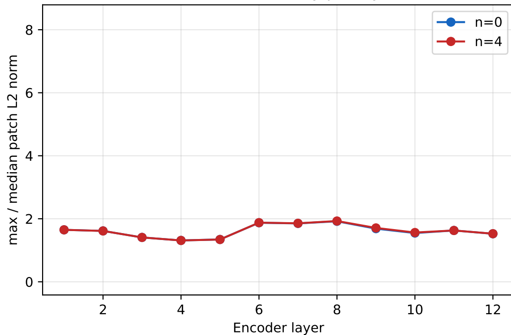
(a) Outlier extremity per layer
