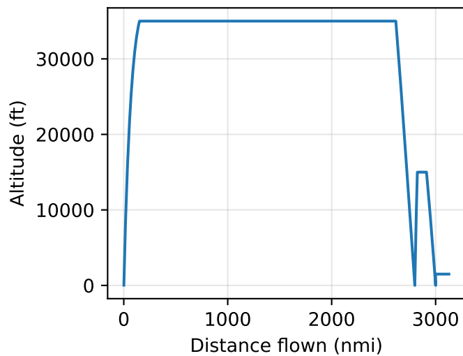
b738 -- openconcept.examples.B738_sizing:B738SizingMissionAnalysis
