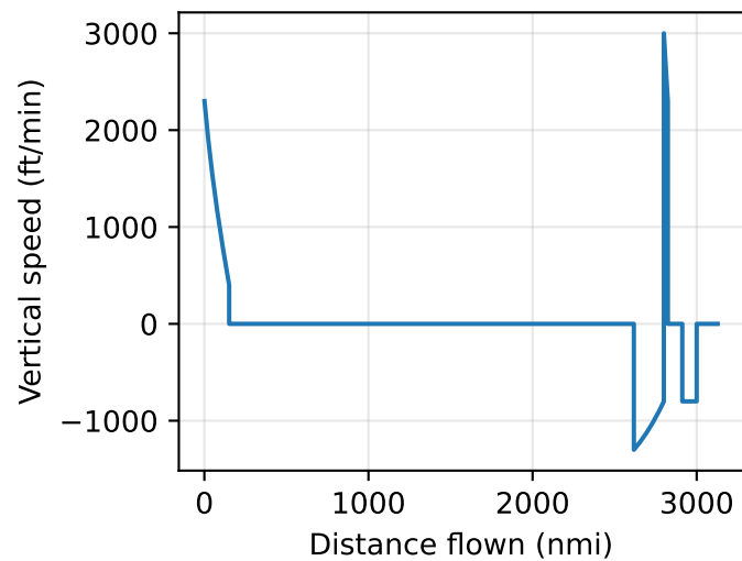
b738 -- openconcept.examples.B738_sizing:B738SizingMissionAnalysis
