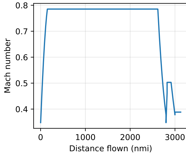
b738 -- openconcept.examples.B738_sizing:B738SizingMissionAnalysis
