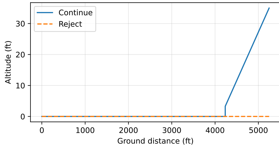
b738 -- openconcept.examples.B738_sizing:B738SizingMissionAnalysis -- balanced field, V1 = 135.1 kn
