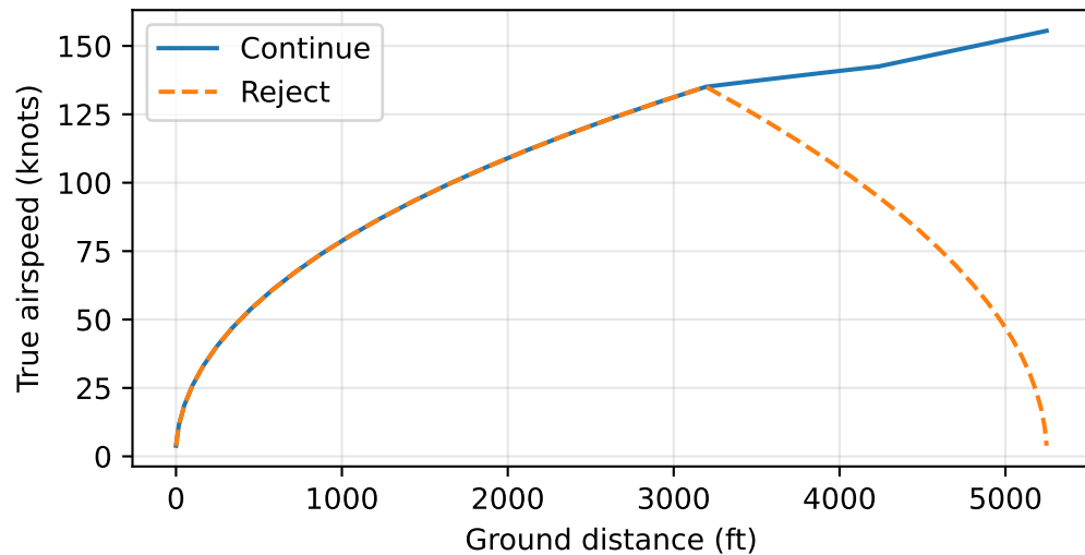
b738 -- openconcept.examples.B738_sizing:B738SizingMissionAnalysis -- balanced field, V1 = 135.1 kn
