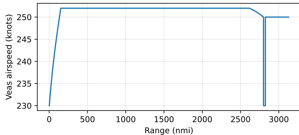
b738 -- openconcept.examples.B738_sizing:B738SizingMissionAnalysis
