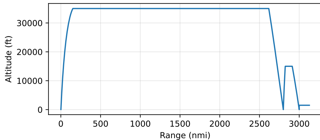
b738 -- openconcept.examples.B738_sizing:B738SizingMissionAnalysis
