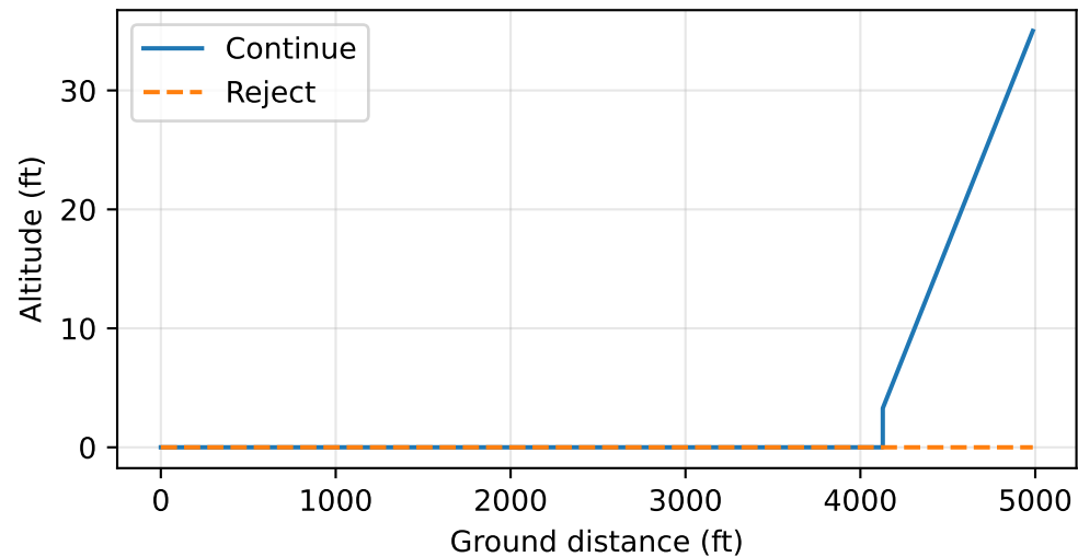
b738_avl -- cdadt.adapter.analysis:SizingMissionAnalysis -- balanced field, V1 = 132.7 kn
