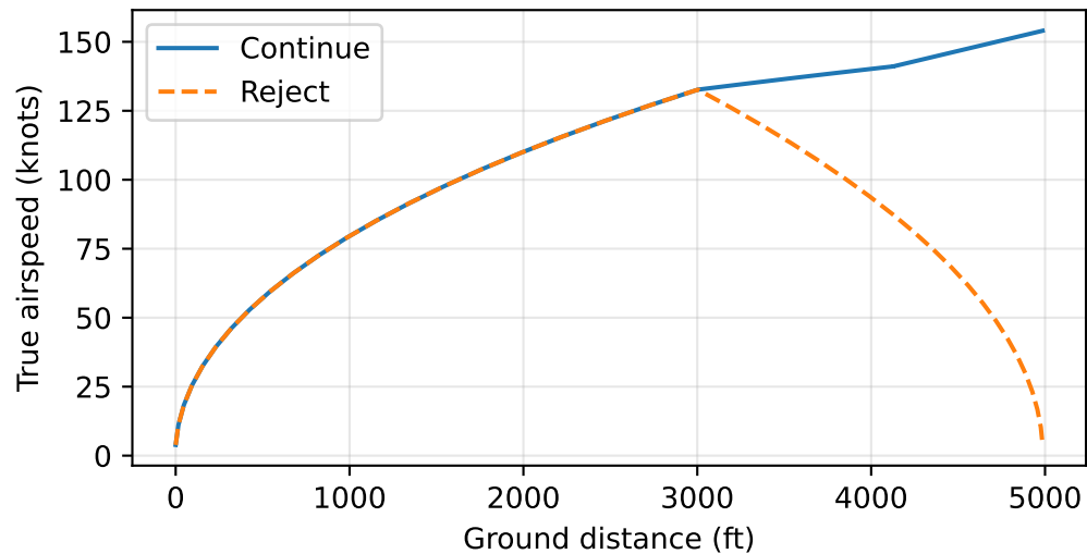
b738_avl -- cdadt.adapter.analysis:SizingMissionAnalysis -- balanced field, V1 = 132.7 kn
