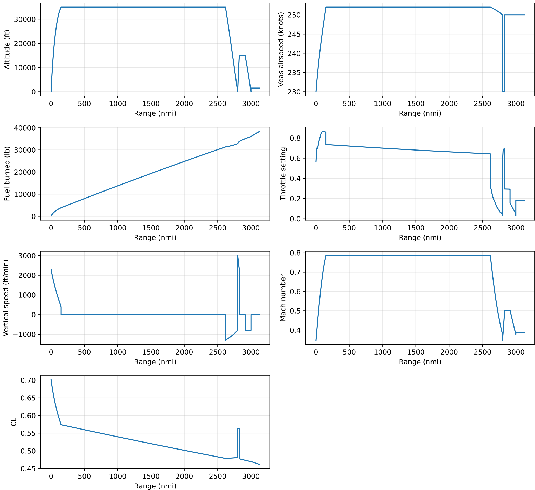
b738_avl -- cdadt.adapter.analysis:SizingMissionAnalysis
