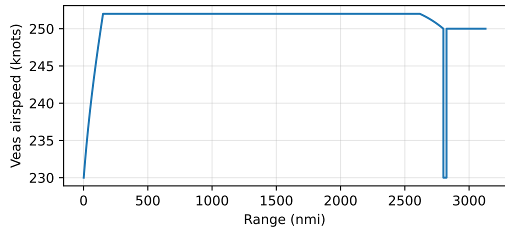
b738_avl_optimization -- cdadt.adapter.analysis:SizingMissionAnalysis
