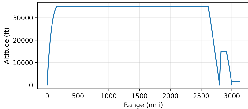
b738_avl_optimization -- cdadt.adapter.analysis:SizingMissionAnalysis
