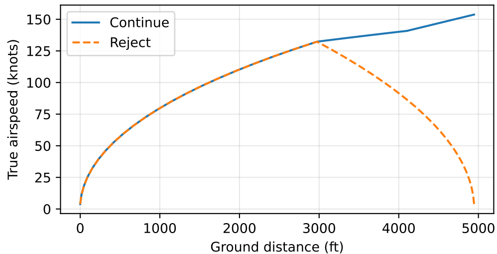
b738_oas -- cdadt.adapter.analysis:SizingMissionAnalysis -- balanced field, V1 = 132.3 kn
