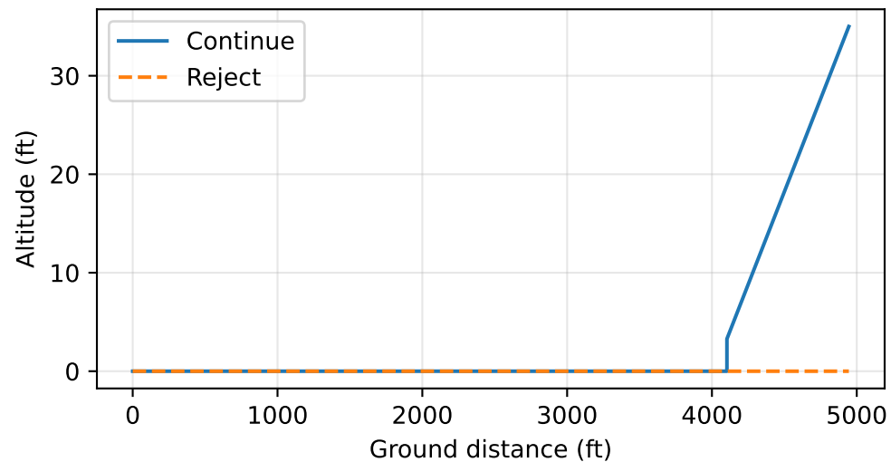
b738_oas -- cdadt.adapter.analysis:SizingMissionAnalysis -- balanced field, V1 = 132.3 kn
