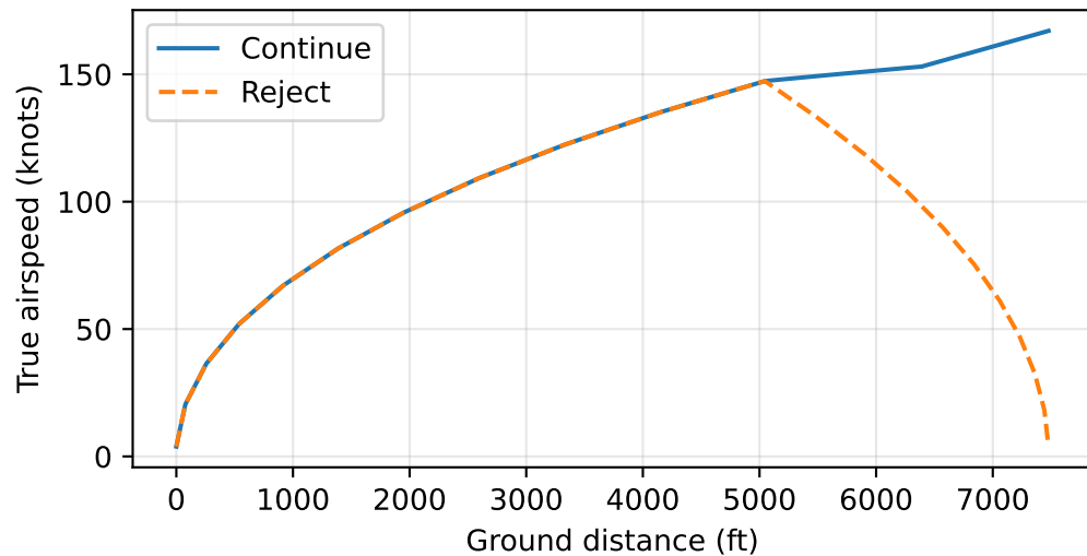
b738_oas_optimization -- cdadt.adapter.analysis:SizingMissionAnalysis -- balanced field, V1 = 147.4 kn
