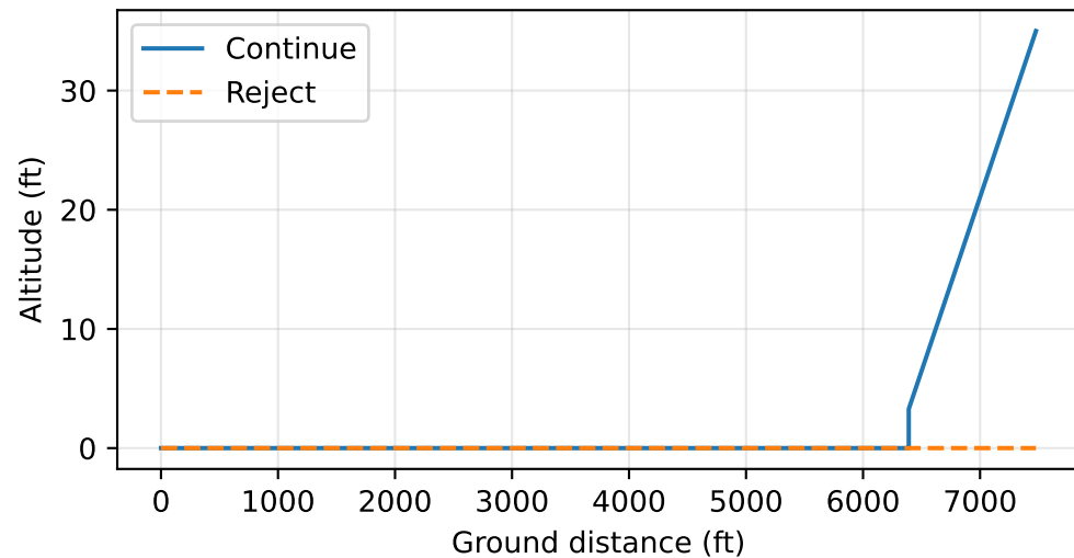
b738_oas_optimization -- cdadt.adapter.analysis:SizingMissionAnalysis -- balanced field, V1 = 147.4 kn
