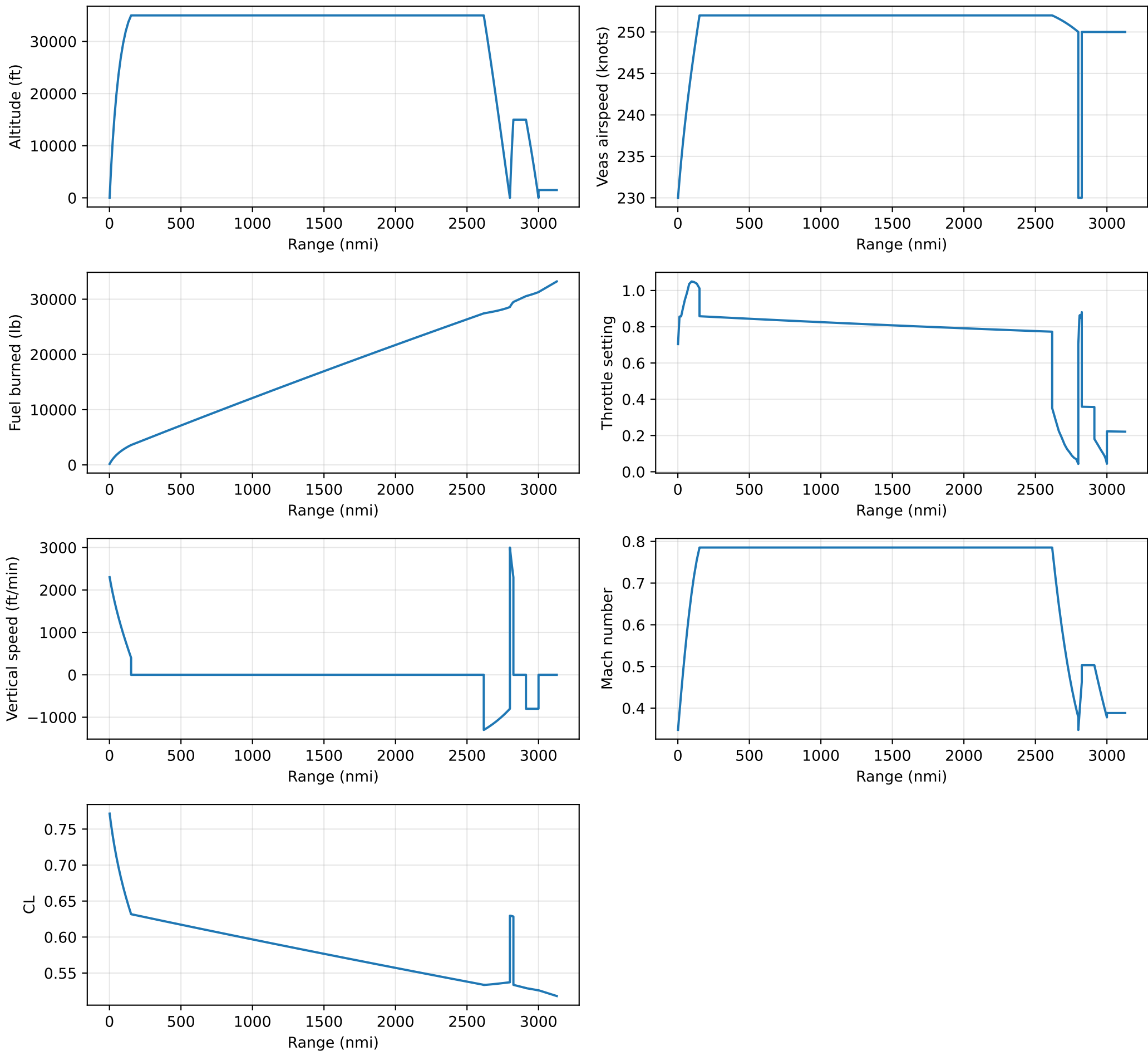
b738_oas_optimization -- cdadt.adapter.analysis:SizingMissionAnalysis
