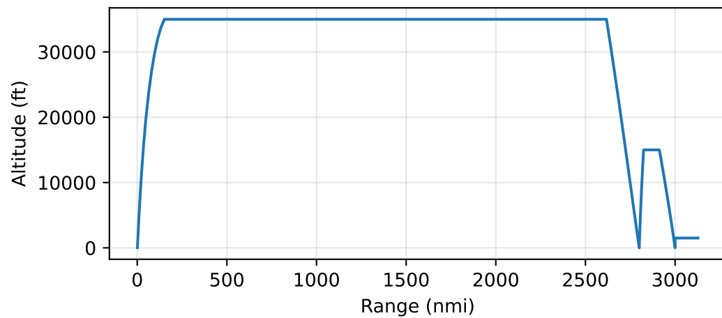
b738_optimization -- openconcept.examples.B738SizingMissionAnalysis
