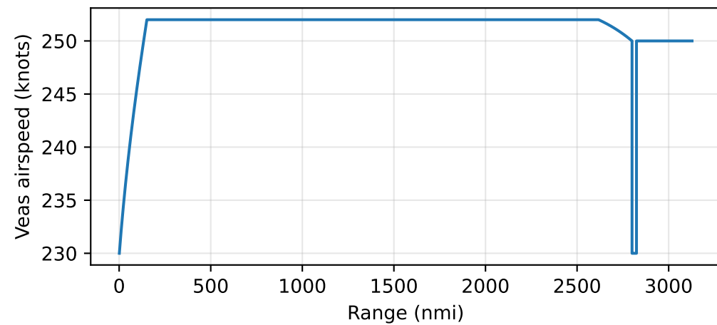
b738_optimization -- openconcept.examples.B738SizingMissionAnalysis
