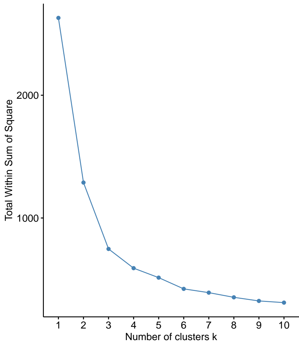
Optimal number of clusters
