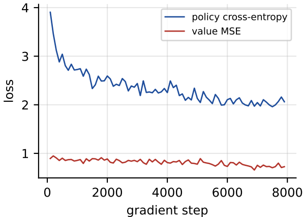
Supervised pretraining (677k positions)
