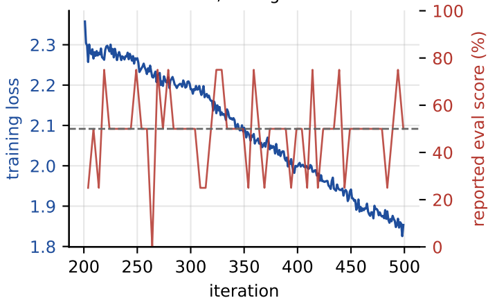
v5: loss falls, strength does not
