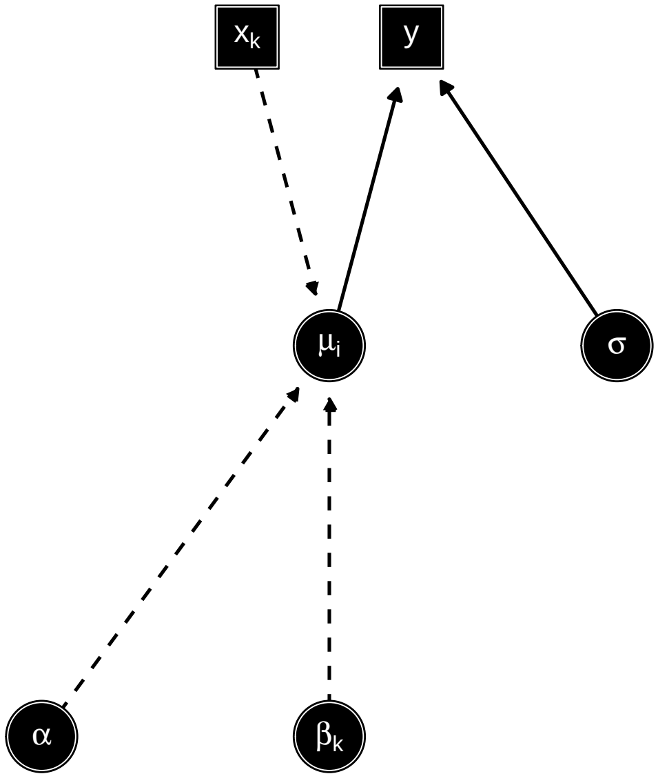
DAG for the Gaussian Linear Regression
