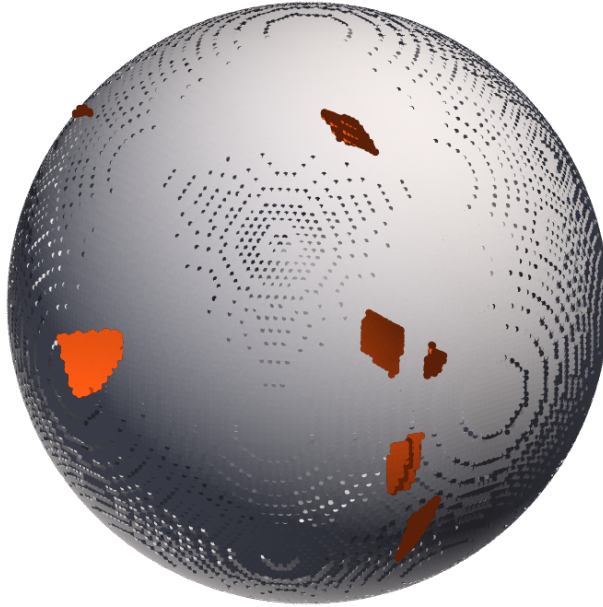
Figure 6: What that silence looks like. The surface is the volume CUDA C++ built at a load factor of 0.283; marked in colour are the points present there and absent from the volume Triton built from identical input. The loss is not scattered, which is the part a count does not convey: it arrives as whole contiguous patches, because the unit that fails to be allocated is a block of 8^3 voxels, and a block that loses its probe takes its entire surface with it. A reconstruction pipeline consuming this would see holes, not noise. On real depth the same failure has a different signature. At a load factor of 0.437 the tartan-dense cell loses 54 blocks scattered across the whole room rather than gathered into a few patches, because real occupancy is irregular where a sphere's is not. That is the harder case to notice: pepper through a reconstruction reads as sensor noise, and a crater does not.
