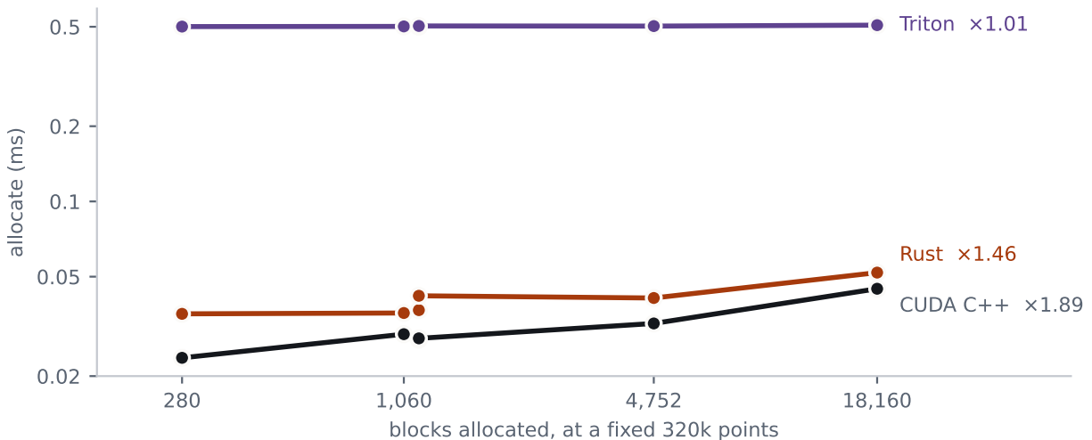
Figure 4: Same points, same launch, different amounts of work. An arm that can leave a probe loop early gets cheaper as the work falls. Triton must run to a compile-time bound, so it does not. The annotation on each line is its spread across the group.
