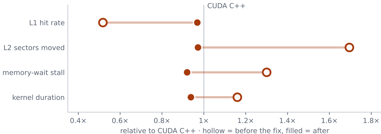
Figure 5: What the two-line change moved, each counter normalised to CUDA C++ so that quantities in different units share one axis. Hollow markers are the Rust kernel before the fix, filled markers after. The kernel was moving 1.70\times the L2 sectors from identical requests and retaining barely half as much in L1; afterwards every counter lands on the reference. Note that for L1 hit rate a value below 1 is the bad direction, since it is the only counter here where more is better.
