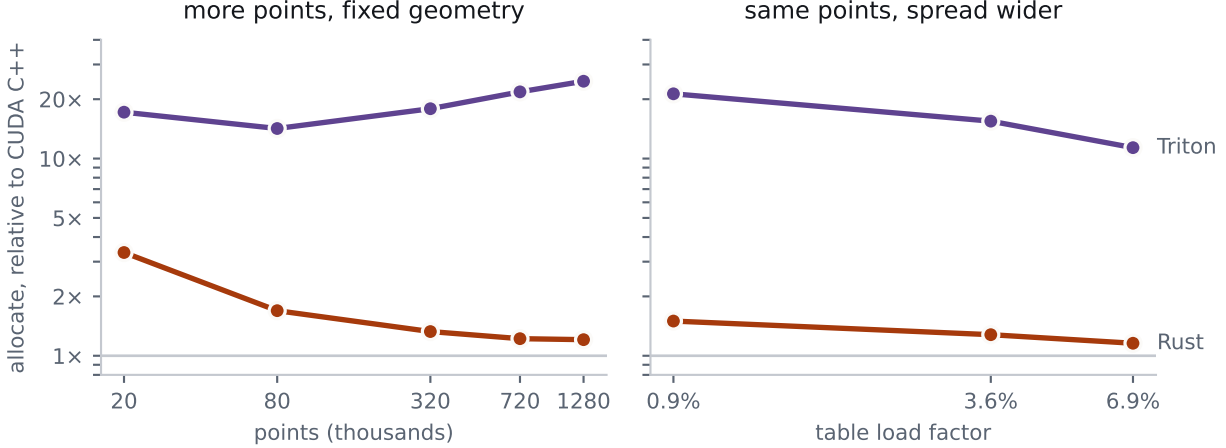
Figure 2: Two levers that move contention in opposite directions, on the RTX 5070 Ti. Adding points over fixed geometry raises the number of threads contending for each table slot, and Triton’s allocate cost rises with it; spreading the same points over more blocks lowers contention, and Triton’s cost falls. A cost driven by problem size would slope the same way in both panels. Rust falls in both, which is the shape of a fixed per-launch cost being amortised rather than a contention cost. Log-log.
