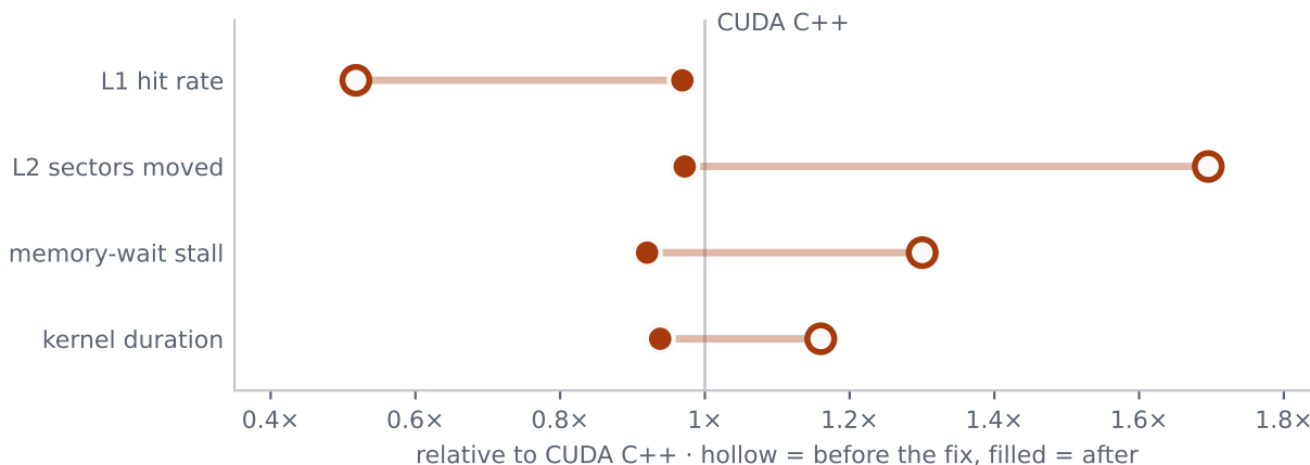
Figure 3: What the two-line change moved, each counter normalised to CUDA C++ so that quantities in different units share one axis. Hollow markers are the Rust kernel before the fix, filled markers after. The kernel was moving 1.70\times the L2 sectors from identical requests and retaining barely half as much in L1; afterwards every counter lands on the reference. Note that for L1 hit rate a value below 1 is the bad direction, since it is the only counter here where more is better.
