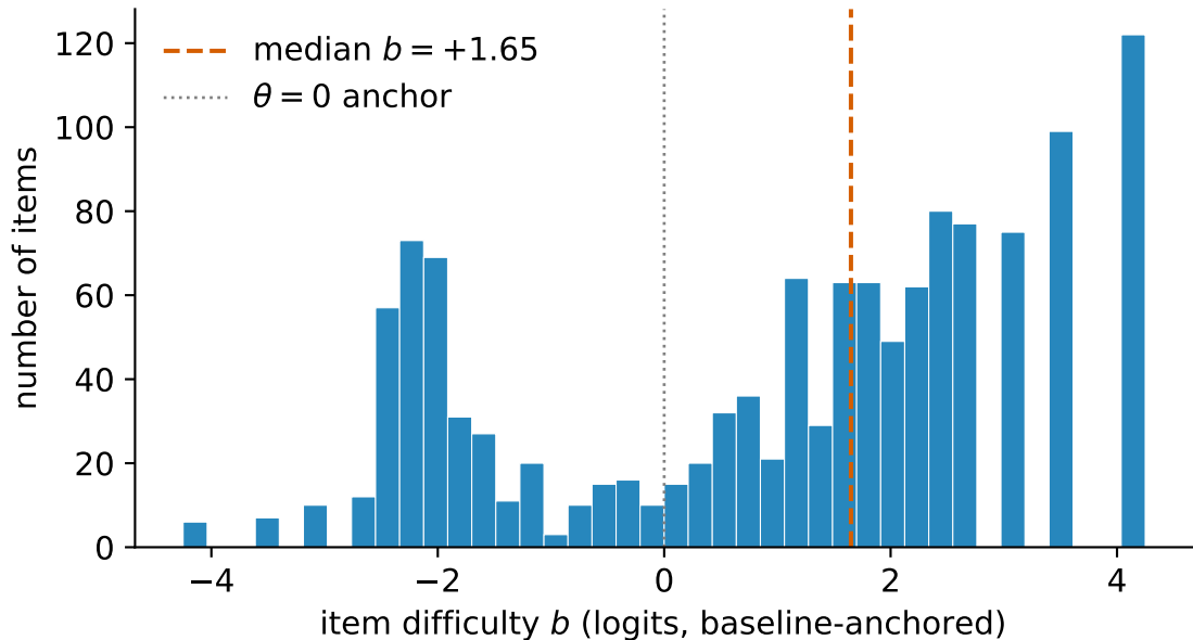
Frozen-bank difficulty distribution ( n = 1284 )
