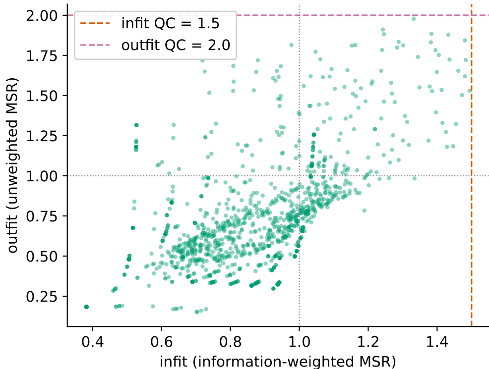
Item fit, frozen bank ( n = 1284 )
