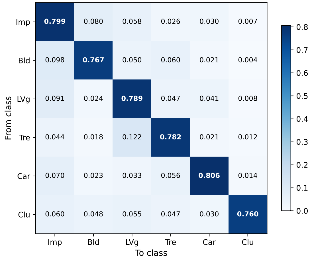
(b) Constrained \alpha \cdot I + (1-\alpha) \cdot R diag ratio: 0.784
