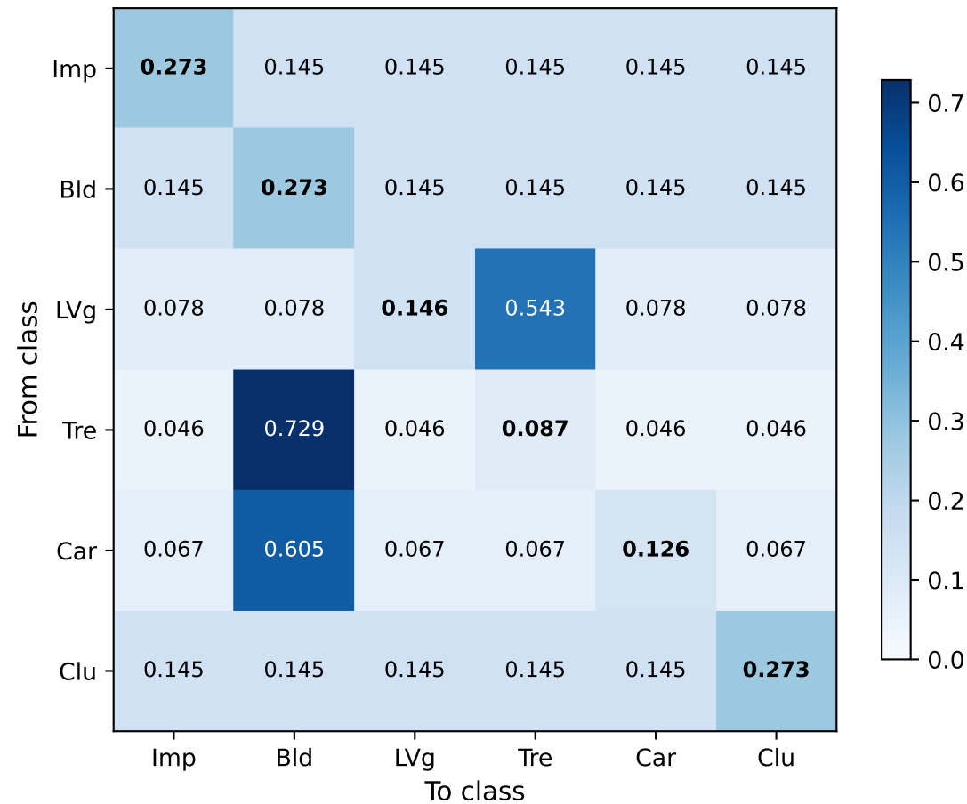
(a) Unconstrained K×K diag ratio: 0.196
