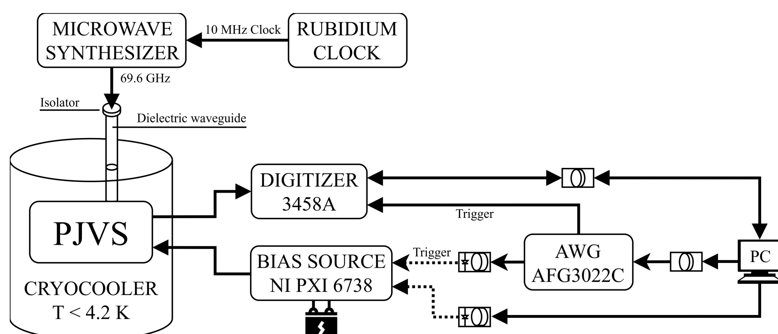
Fig. 1 – Experimental setup
