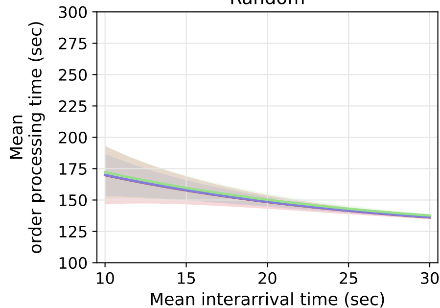
Random
