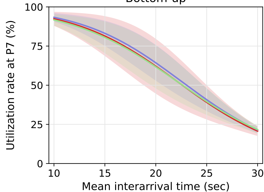
Bottom-up
