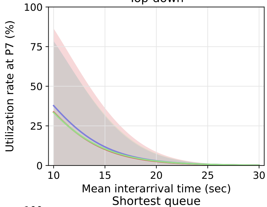
Top-down
