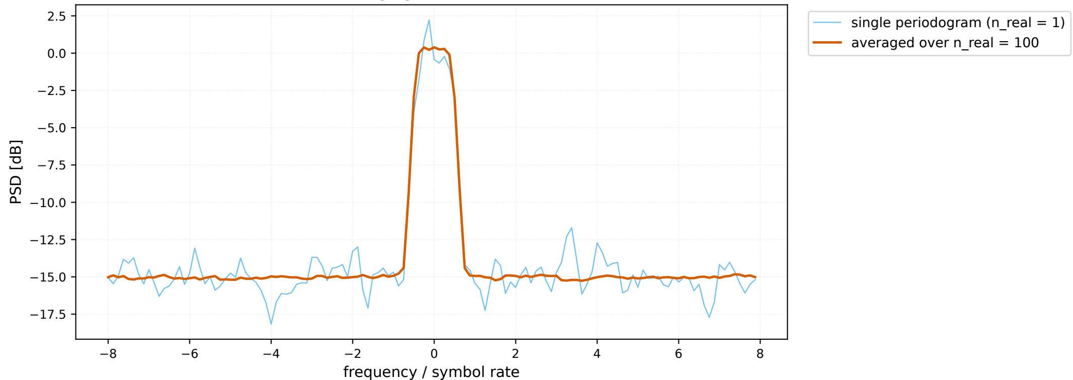
Effect of ensemble averaging on H1 PSD estimate ( a_3 = -0.32 )
