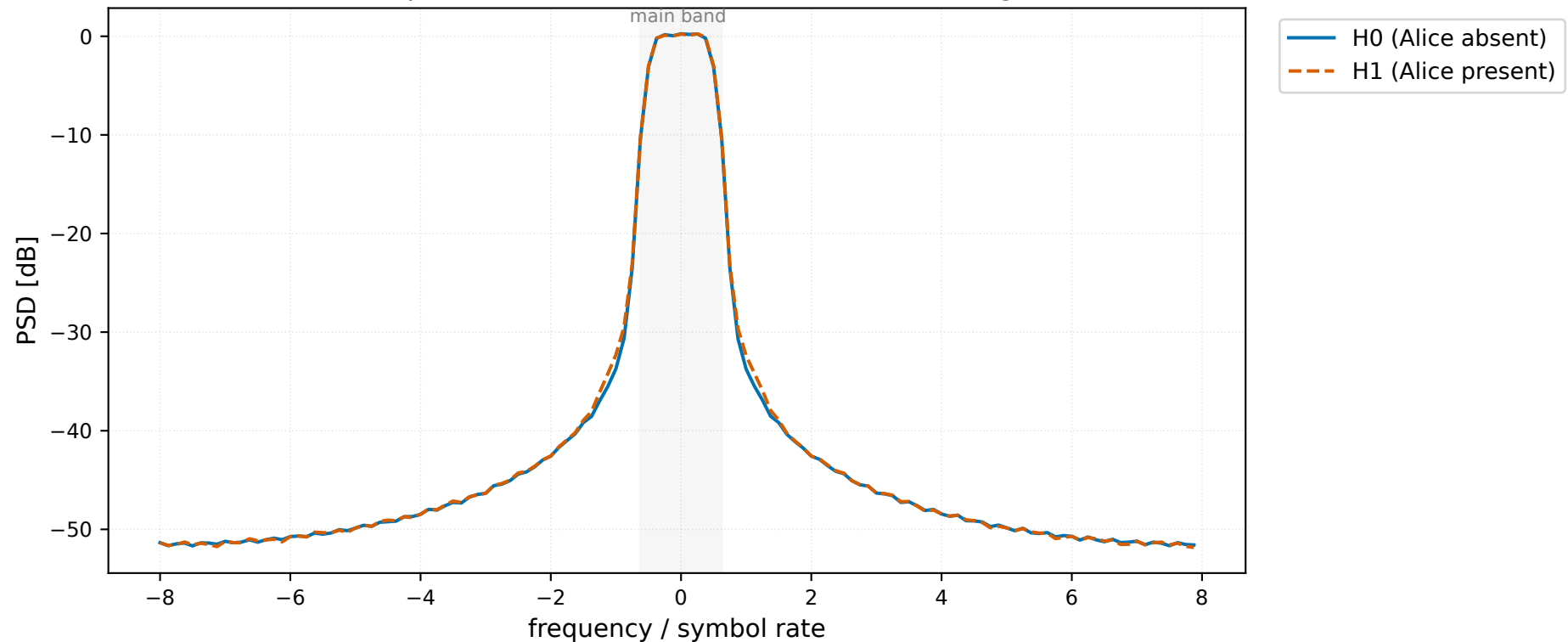
H0 vs. H1 PSD after unit-power normalization (a3 = -0.32, Welch avg of 200 realizations)
