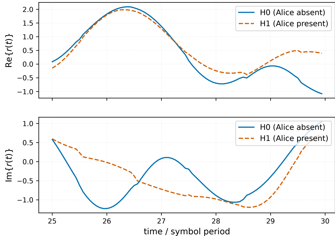
H0 vs. H1 received baseband signal ( a_3 = -0.32 )
