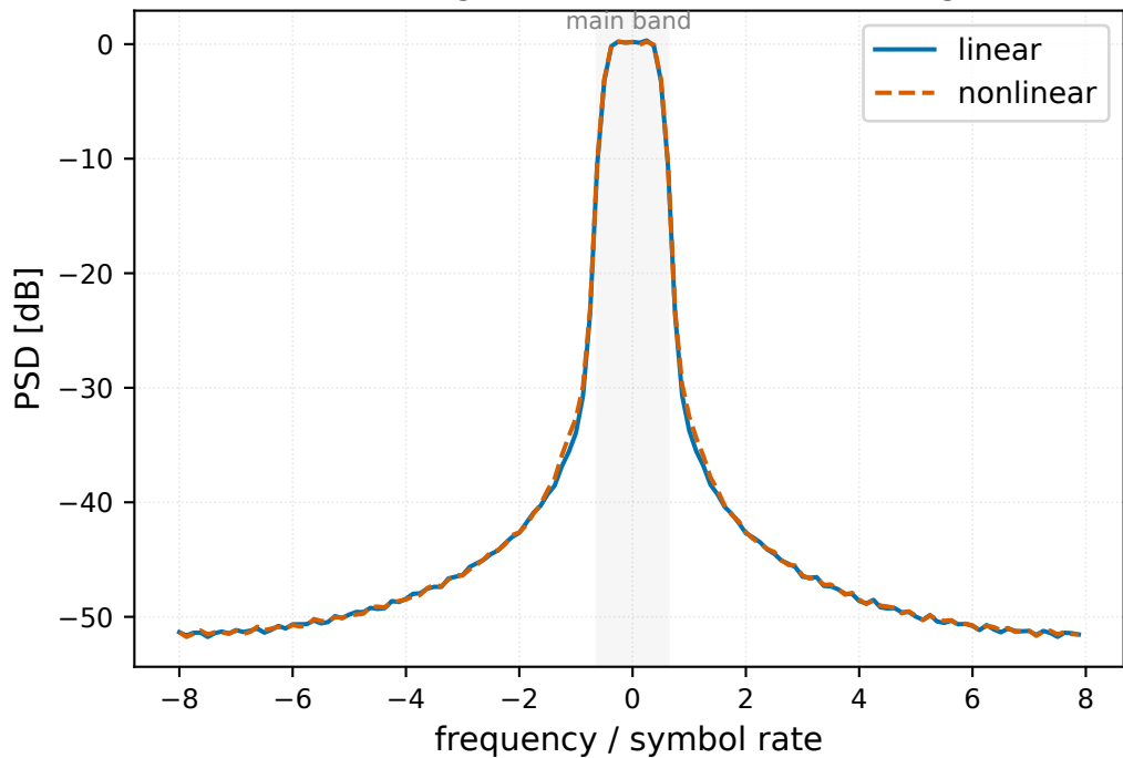
PSD of linear vs. nonlinear signal ( a_3 = -0.32 , Welch avg of 200 realizations)
