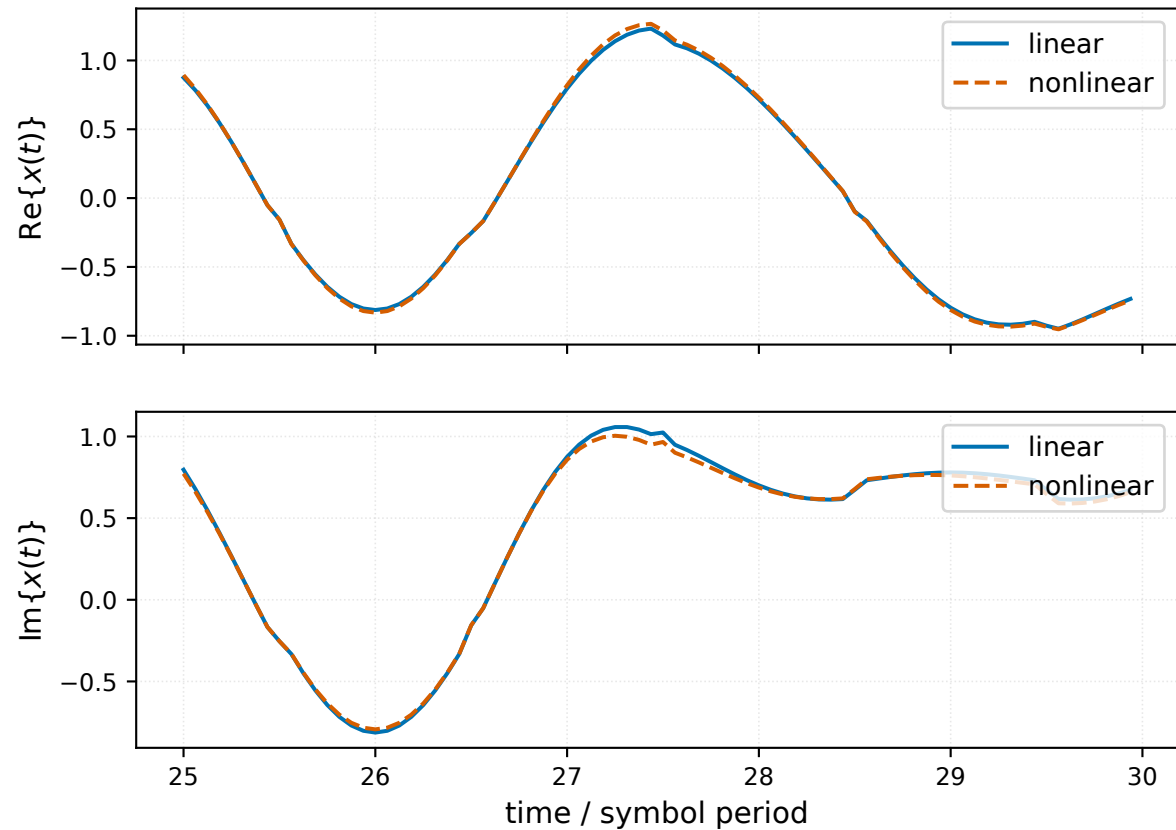
Linear vs. nonlinear baseband signal ( a_3 = -0.32 )
