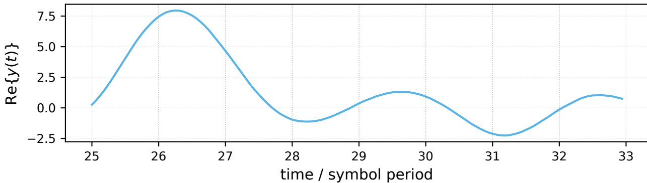
(c) Matched filter output (dotted lines: symbol-decision instants)
