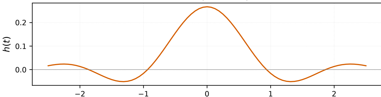
(b) Matched filter impulse response (SRRC)
