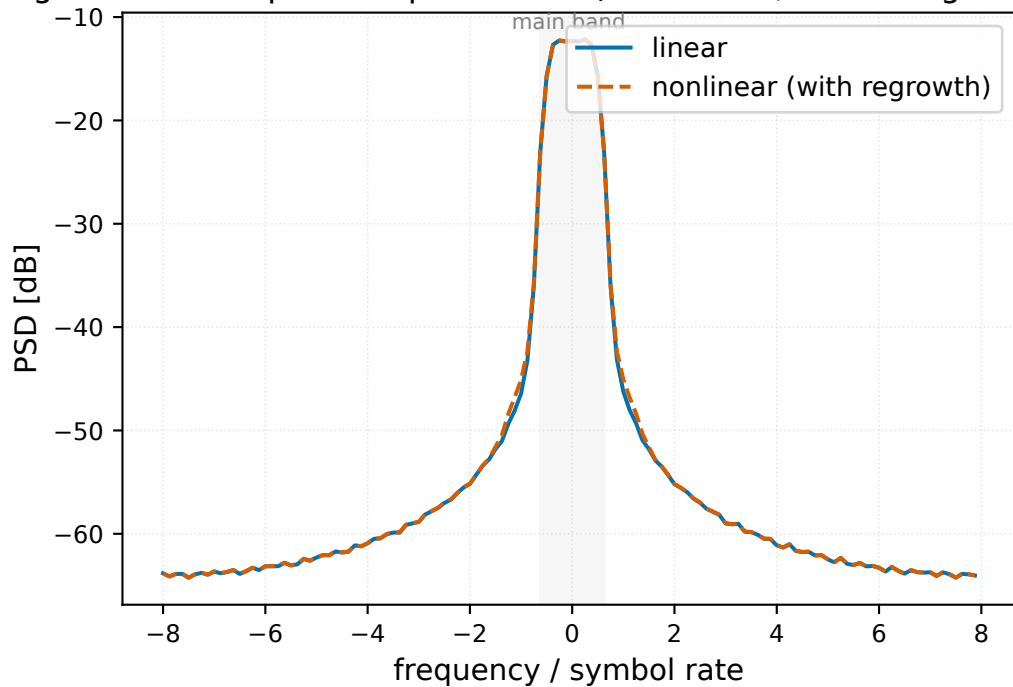
Spectral regrowth before power equalization ( a_3 = -0.32 , Welch avg of 200 realizations)
