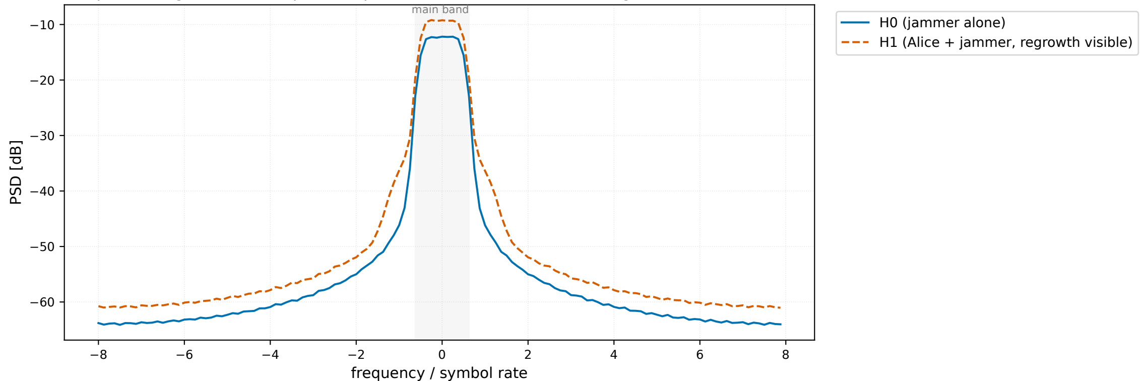
Spectral regrowth before power equalization ( a_3 = -1.0 , Welch avg of 200 realizations)
