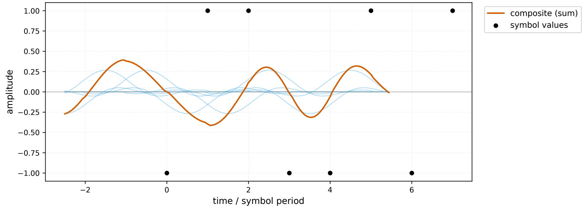
Pulse train: individual SRRC pulses (light) summing to the transmitted waveform
