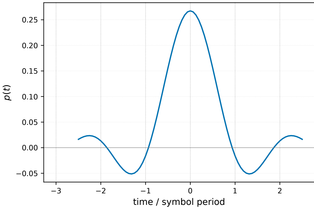
SRRC pulse ( \beta = 0.25 , span = 5 symbols)
