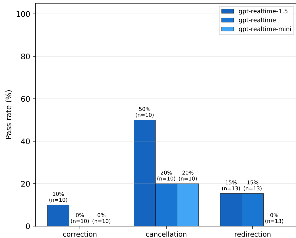
(a) Speech-phase (intra-turn) interruption (total 33 tasks)
