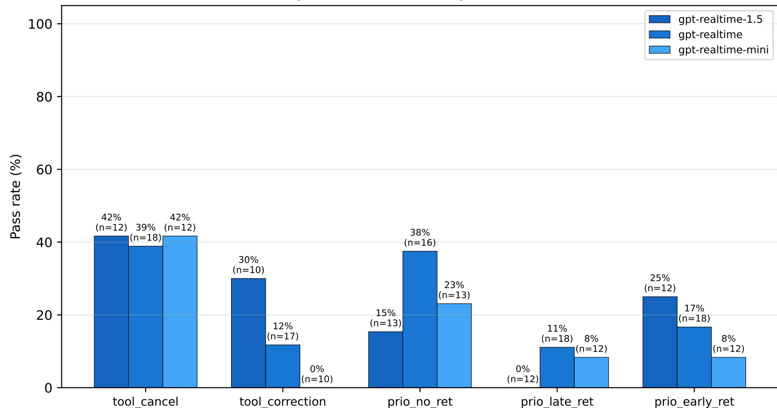
(b) Tool-phase (inter-turn) interruption (total 87 tasks)
