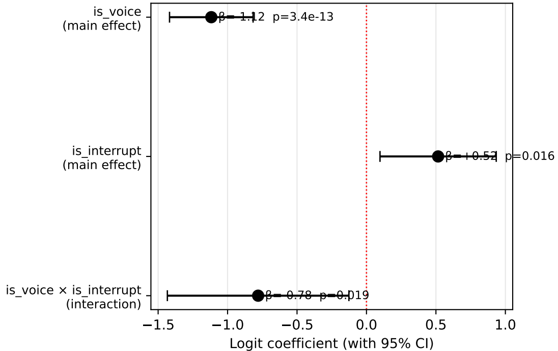
Logistic regression coefficients (passed \sim is_voice \times is_interrupt)
