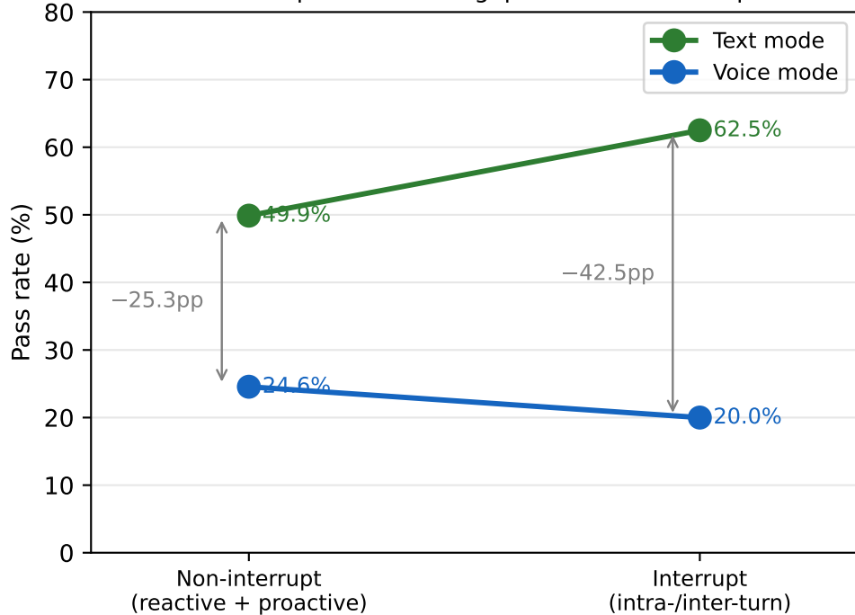
Voice × Interrupt interaction: gap widens on interrupt tasks
