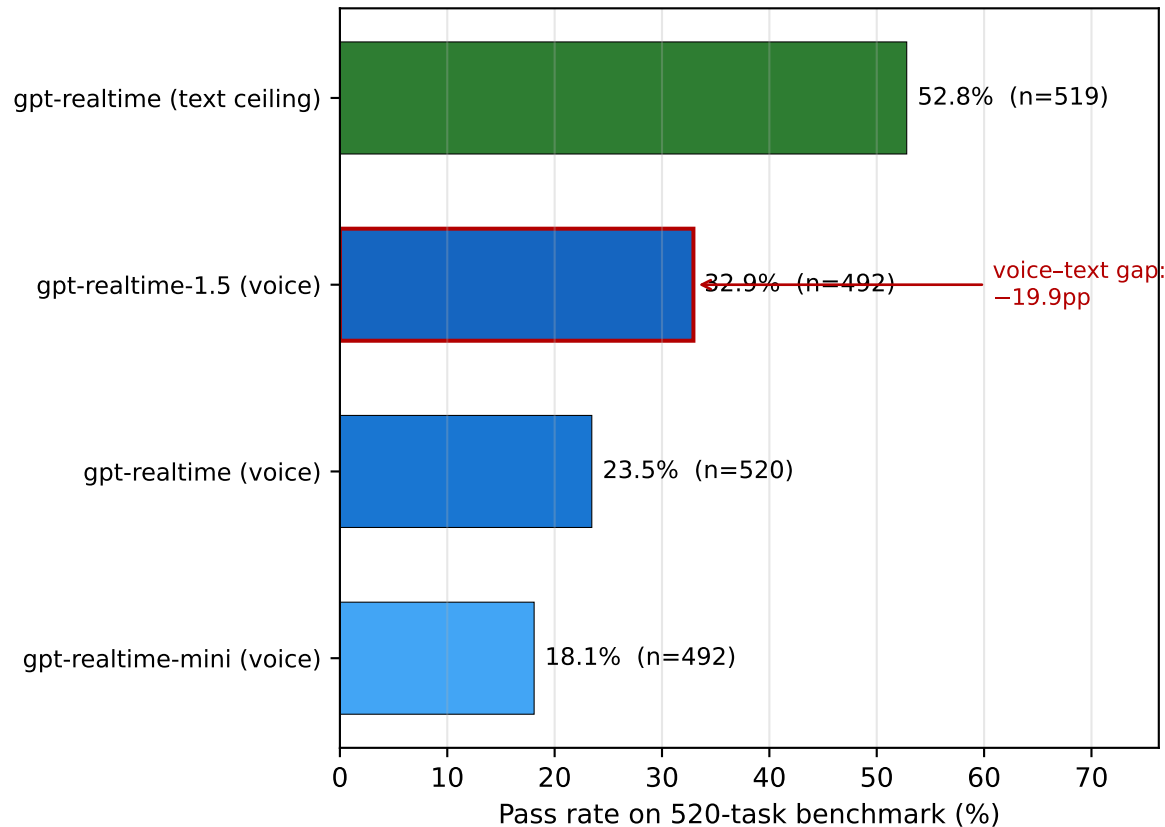
(a) gpt-realtime family on audio tool-calling benchmark (520 matched tasks; text baseline = input_mode="text" ceiling)
