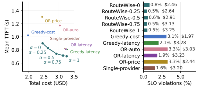
Figure 1. Cost–latency trade-off on a 24-hour BurstGPT replay of MiniMax-M3. (Left) Total serving cost versus TTFT; lower left is better. Routewise provides a control knob to balance between cost and latency. (Right) Fraction of requests exceeding the 3-second TTFT target; labels give total cost. Greedy-cost and Greedy-latency optimize one objective; OR-auto, OR-price, and OR-latency are OpenRouter routing modes [33], and Single-provider sends every request to the best on-demand provider.
