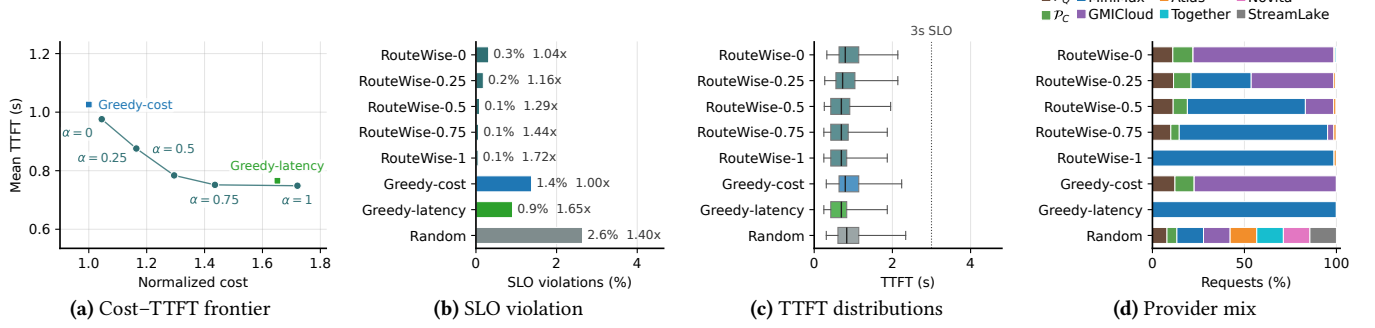
Figure 10. Thirty-day BurstGPT simulation. Costs in (a) and the \times labels in (b) are normalized to Greedy-cost. Boxes show the interquartile range and median; whiskers span the 5th–95th percentiles.
