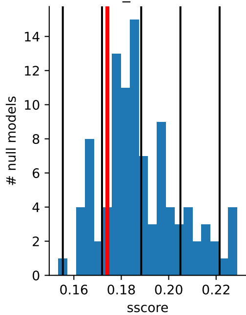
ss_z: -0.86
