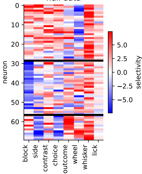
ss_z: -0.86
