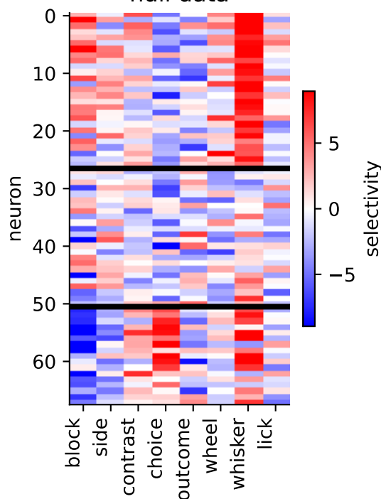
ss_z: 1.11
