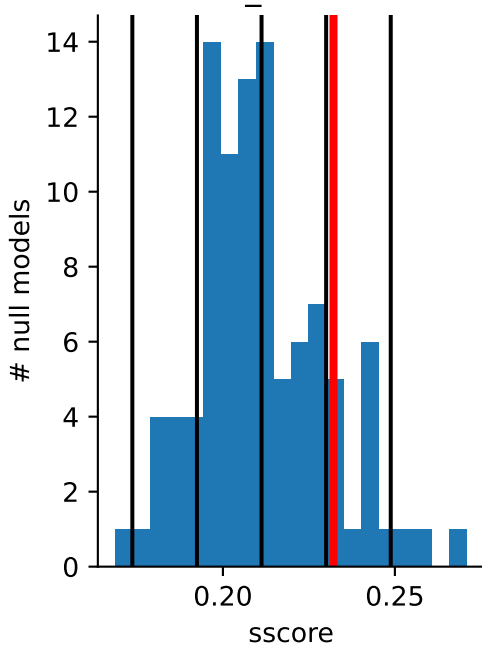
ss_z: 1.11
