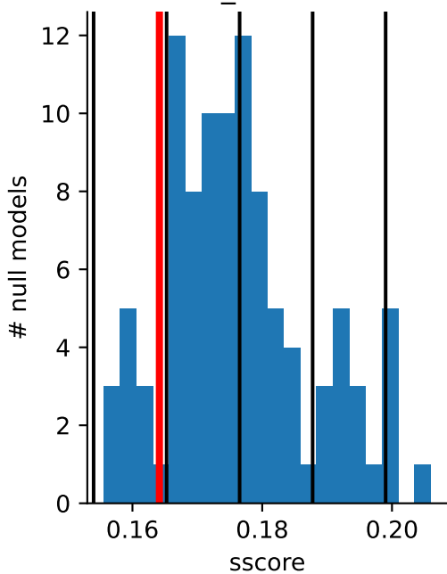
ss_z: -1.10
