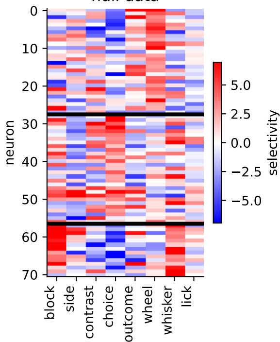
ss_z: -1.10
