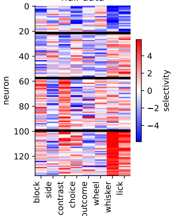
ss_z: 1.70
