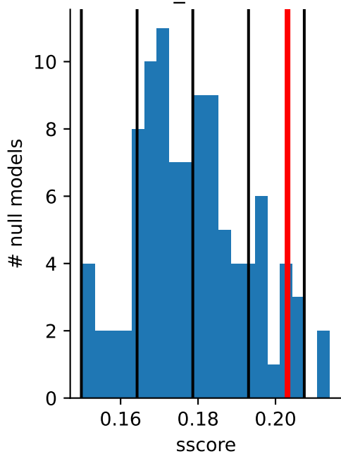
ss_z: 1.70
