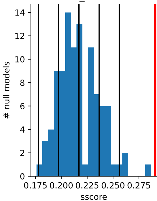
ss_z: 3.76
