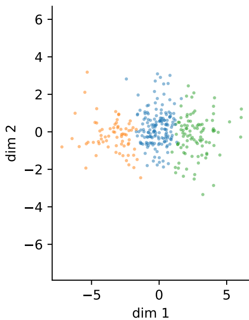
lda
