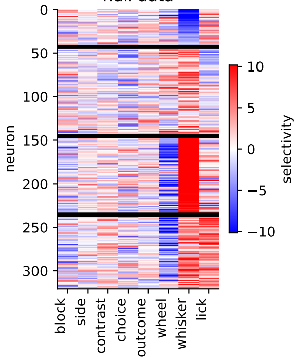
ss_z: 2.31
